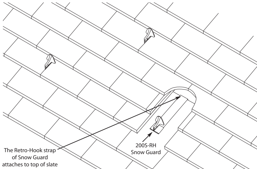
Typical Snow Guard spacing on 1/4" (.025") thick slate.
